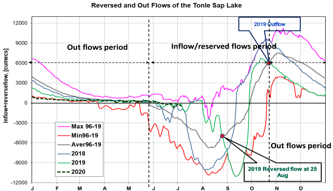
Figure 5 The seasonal change of inflows and outflows of the Tole Sap Lake
