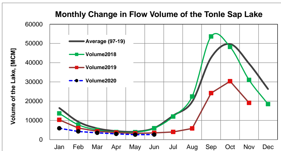
Figure 5 The seasonal change in monthly Volume Flows of the Tole Sap Lake up to June 2020
