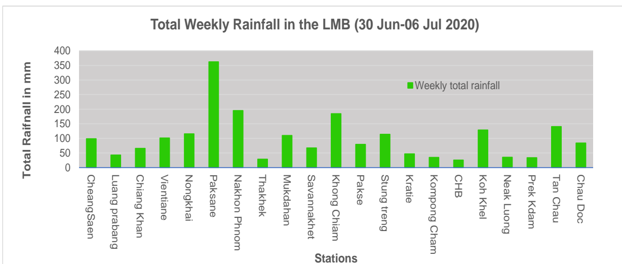
Figure 3 Daily accumulated rainfall over the LMB
