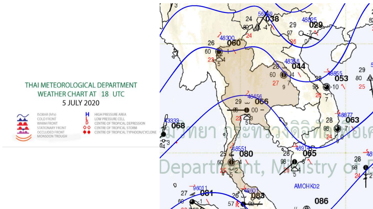
Figure 1 Summary of weather condition over the LMB on 06 July 2020
