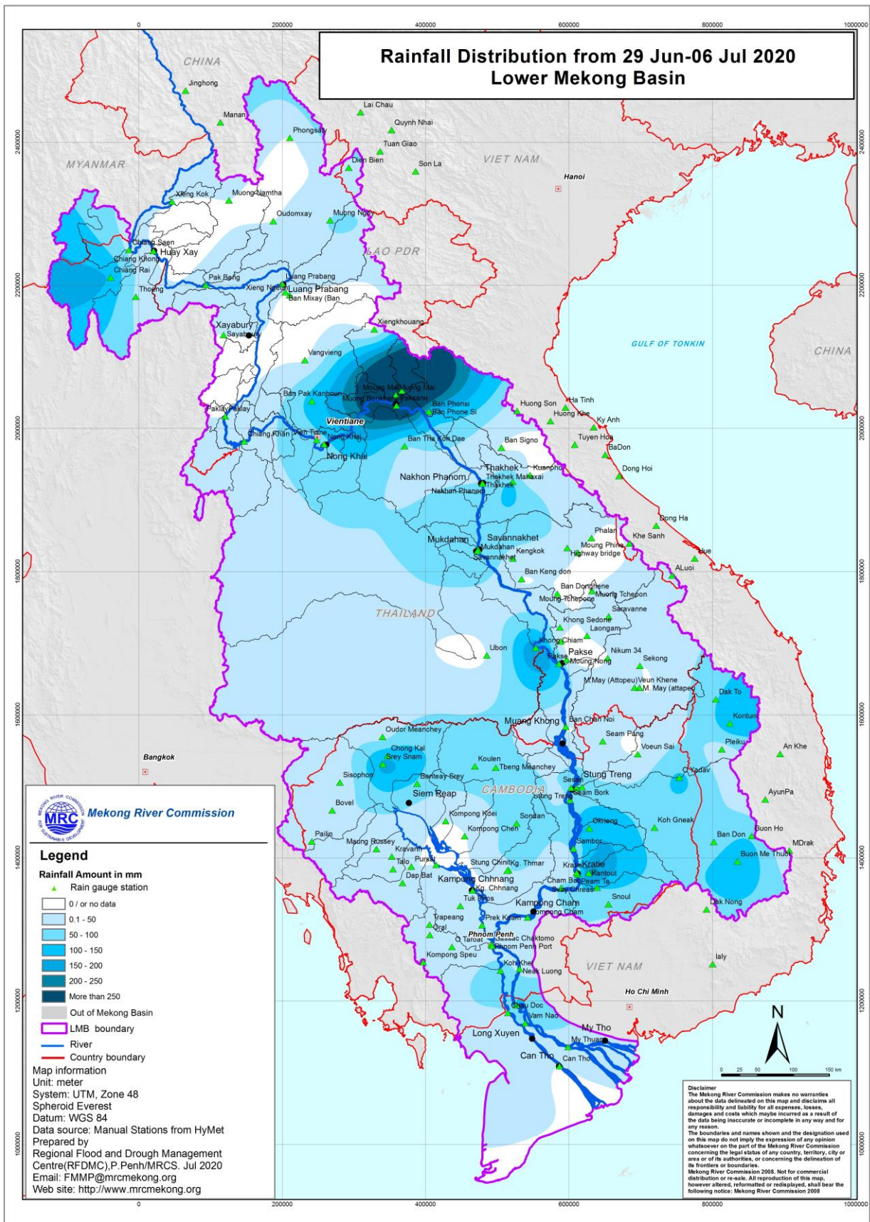
Figure 4 The weekly rainfall distribution from 29 June to 06 July 2020 over the LMB
